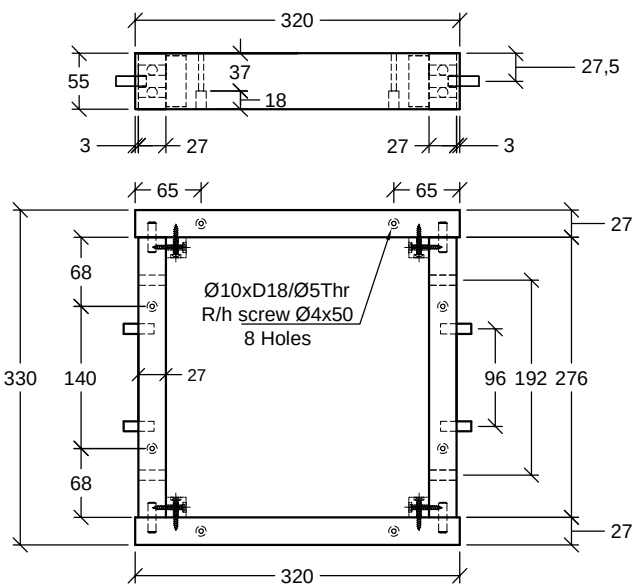
APRON FRAME RUBBER WOOD 1 PC/SET
